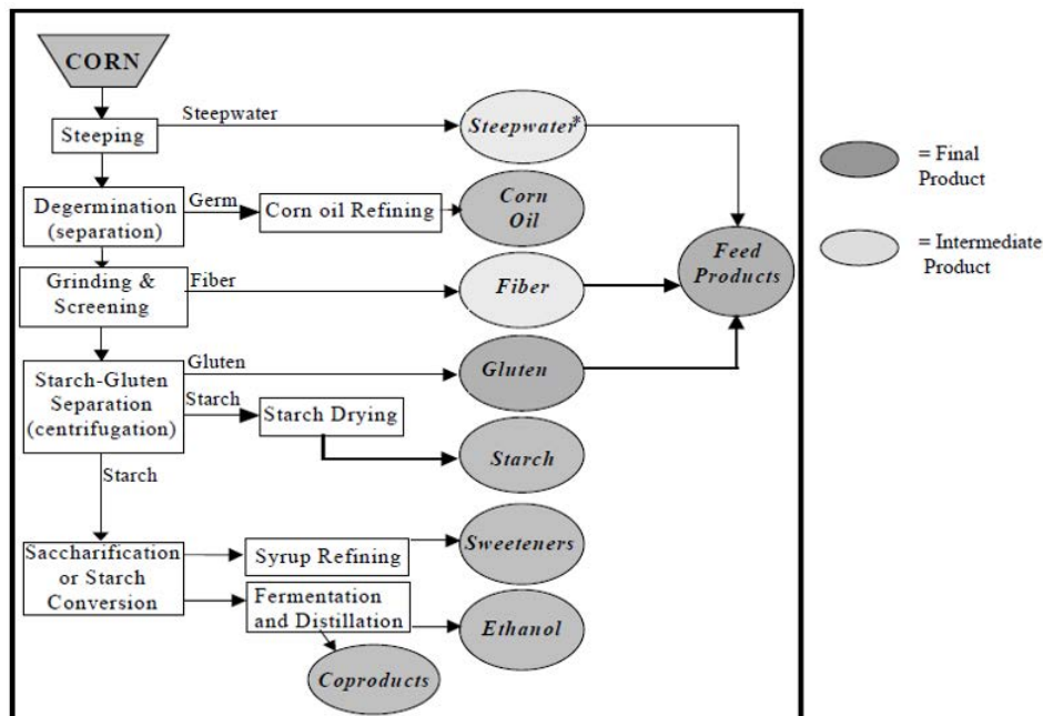
Figure 54. Overview of the processes and products of wet corn milling (Galitsky et al., 2003)
