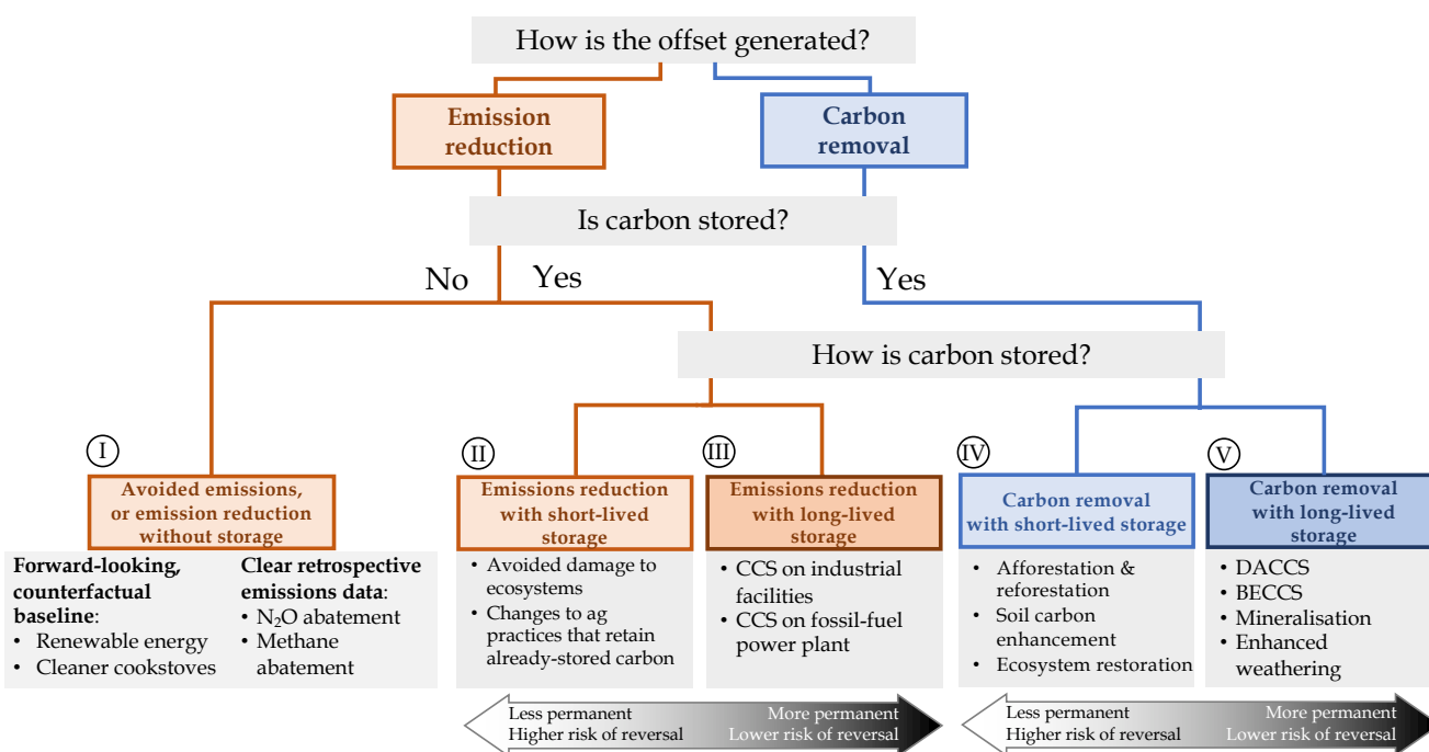
Figure 1 - This simplified classification scheme shows five types of carbon offset based on whether carbon is stored, and the nature of that storage. Carbon removal is defined as the act of taking CO 2 out of the air and permanently storing it. For all forms of carbon removal, whether nature-based solutions or technologically-mediated processes, carbon must be stored. Principle 2 addresses the distinction between emission reduction and carbon removal. For offsets that involve storing carbon, a further distinction is made as to whether that storage is likely to be short-lived (on the order of decades) or long-lived (on the order of centuries to millennia). Principle 3 addresses the distinction between short-lived and long-lived storage. Note that avoided emissions (Type I) should not be considered superior to Types II-V on the basis of permanence, since such emissions may only be temporarily avoided. The marginal quantity of fossil fuel whose use is avoided by such an offset might get purchased and consumed by someone else (carbon leakage), or it may remain in the ground for years, only to be extracted and emitted at a later date when prices and other conditions change (intertemporal carbon leakage). Avoided emissions can therefore also suffer from poor “permanence” if the reduction is not enduring. Figures 1 & 2 prepared by Eli Mitchell-Larson.
