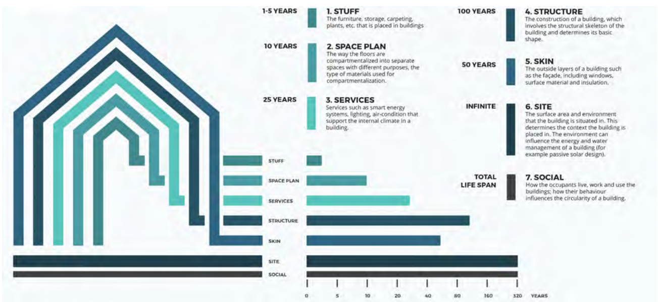
Figure 5: Building model consisting of the building related layers based on the sharing layers 9
